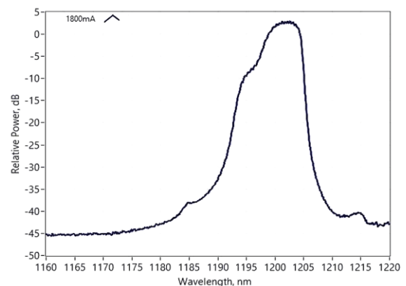
Emission Spectra
