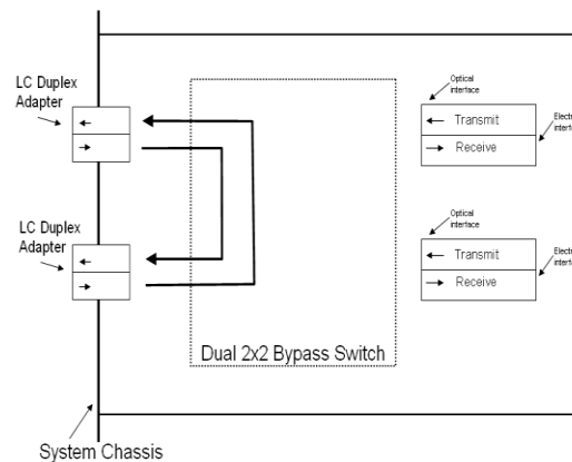
Bypass Mode
