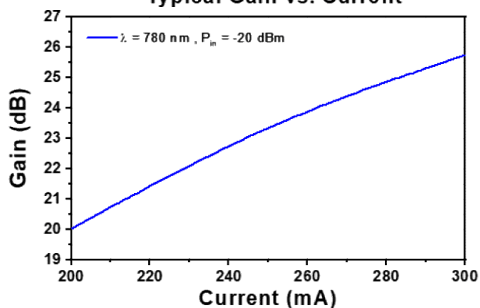
Typical Gain vs. Current
