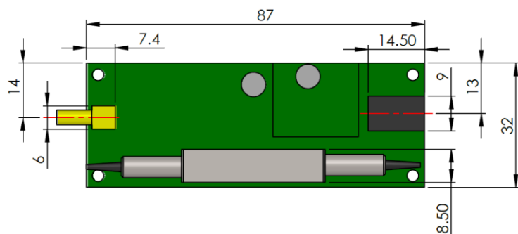
Back view
