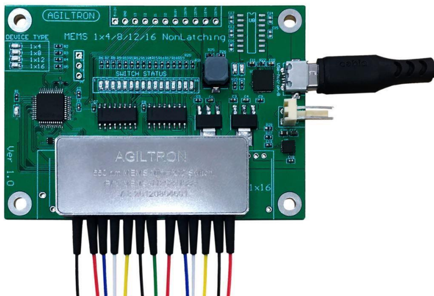
MEMS-1x12 on Demo driver
