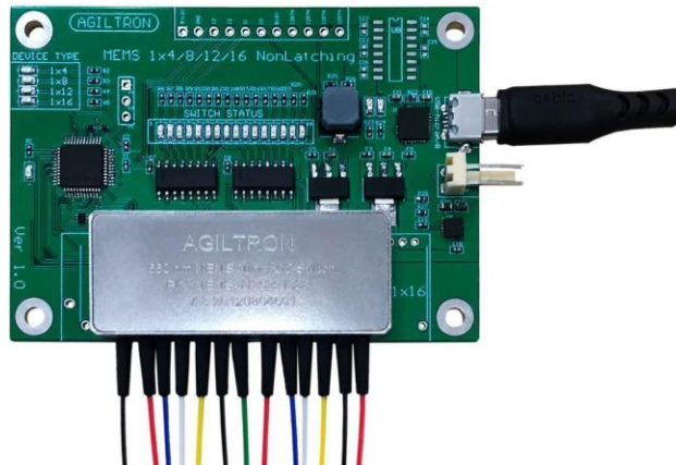
MEMS-1x12 on Demo driver
