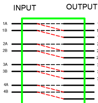
Quad 2x2 Bypass
