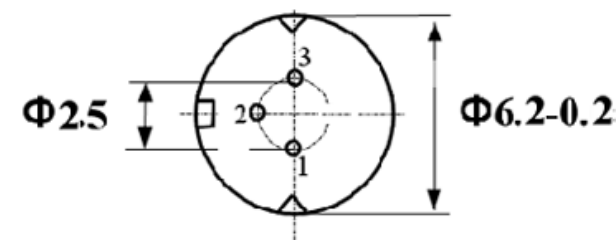
Bottom View
