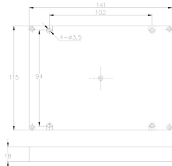
Package 4: 18x115x141 (HxWxL) mm
