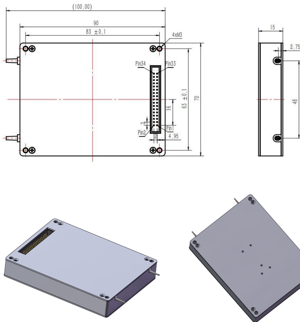
Figure 1 Mechanical drawing
