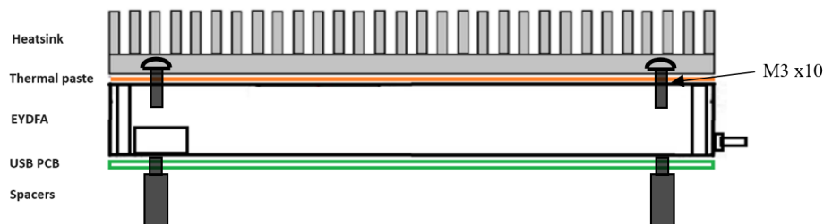
Figure 2 Heatsink installation
