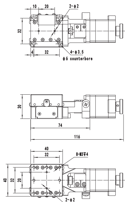
CXPF30-80
