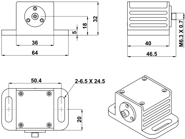
SLE-S mounting and connector dimensions in millimeters.
