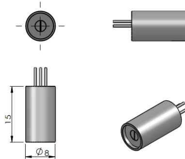
Dimensions of PCB1( small size , 9 \times 12\text{mm}^2 , 6V)
