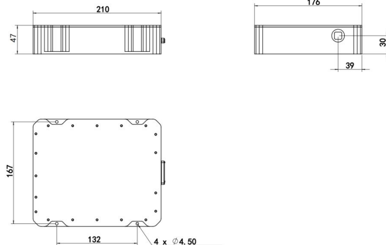
LASER HEAD (OEM-BD-455) 1
