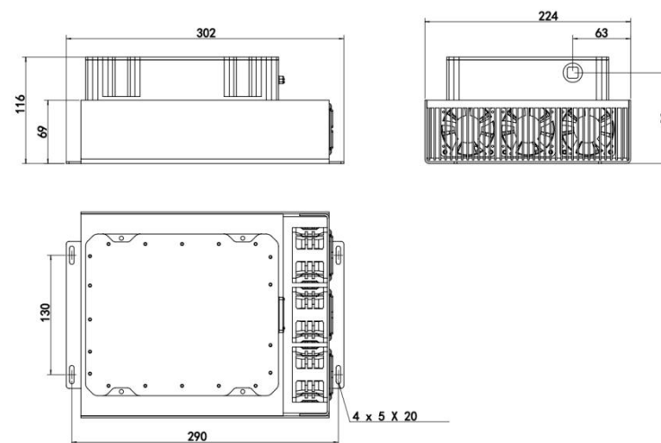
LASER HEAD (BD-455-HS)
