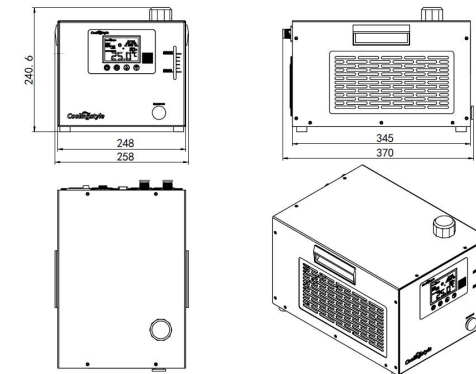
Water Chiller(WCH-580)
