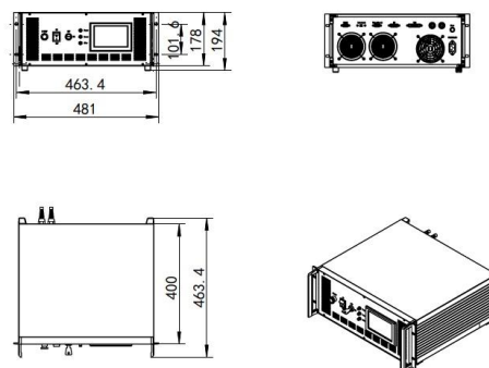
PSU-AOM (4U)
