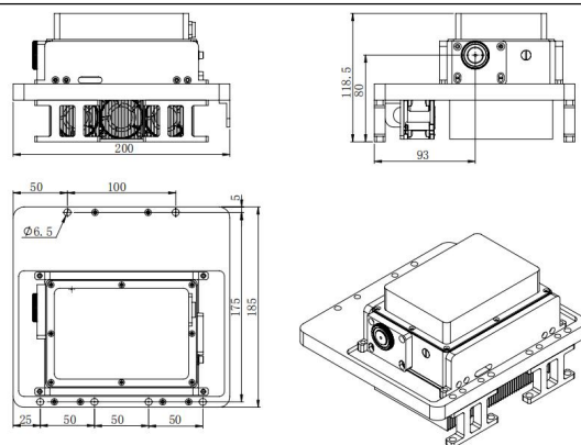
LASER HEAD (EO-532-N-I) 4
