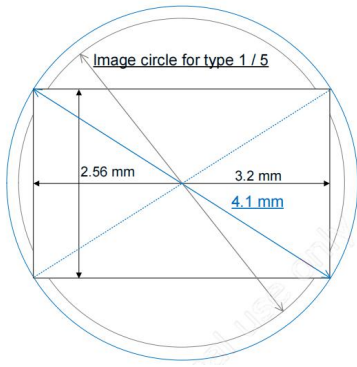
Figure 9 IMX991 relationship between image circle and pixel area
