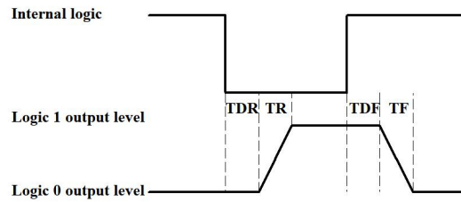
Figure 49 Output logic levels
