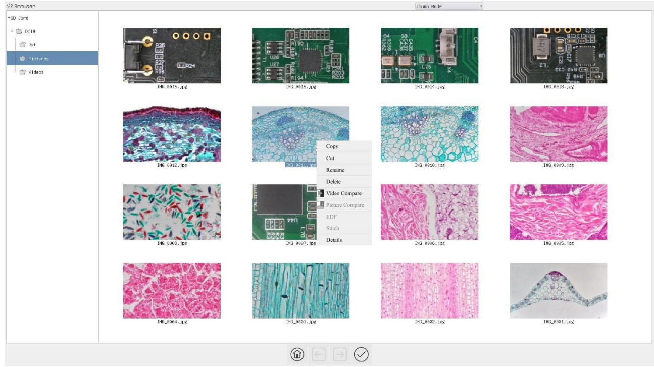
Figure 23 Browsing UI
