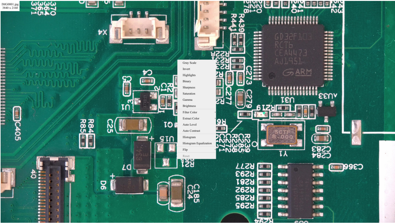
Figure 24 Image Processing
