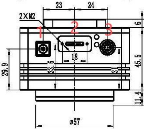
Figure 12-16 CTR3CMOS Camera interface diagram
