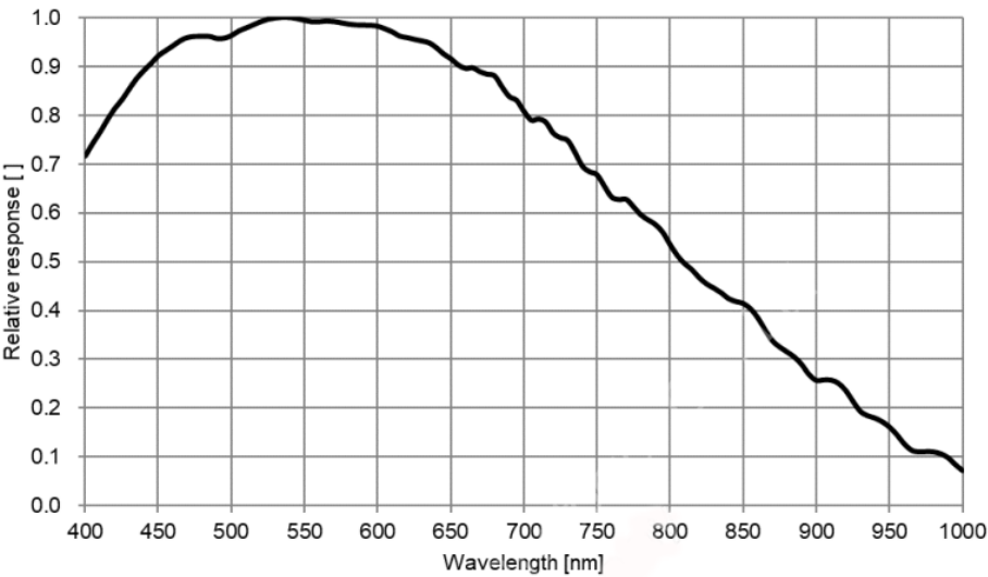
Figure 6-29 IUA5100KMA spectral response curve
