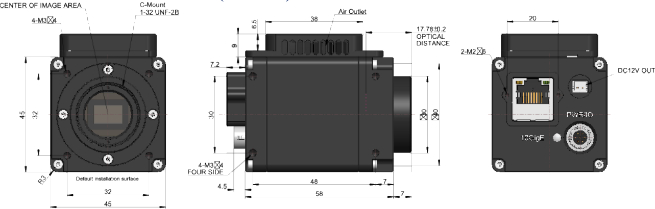
Figure 12-25 Dimensions of camera housing(mm)
