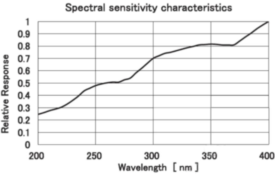
Figure 6-86 IUA8000KMA spectral response curve
