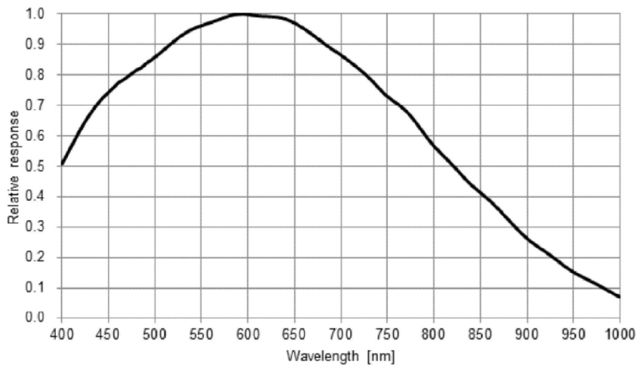
Figure 5-88 I3CMOS12300KMA spectral response curve
