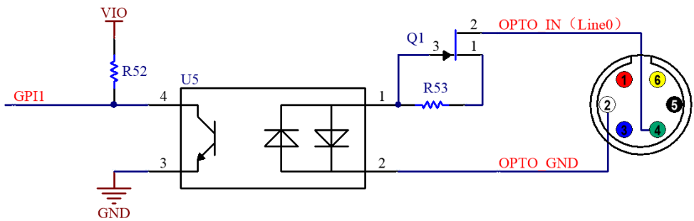
Figure 13-9 Opto-isolated input circuit
