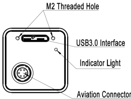
Figure 12-22 Schematic diagram of camera back panel
