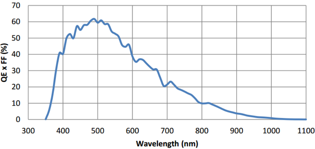
Figure 7-3 IUB43000KMA spectral response curve
