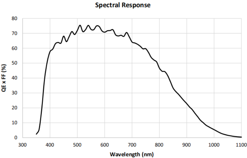
Figure 5-73 I3CMOS05100KMA spectral response curve
