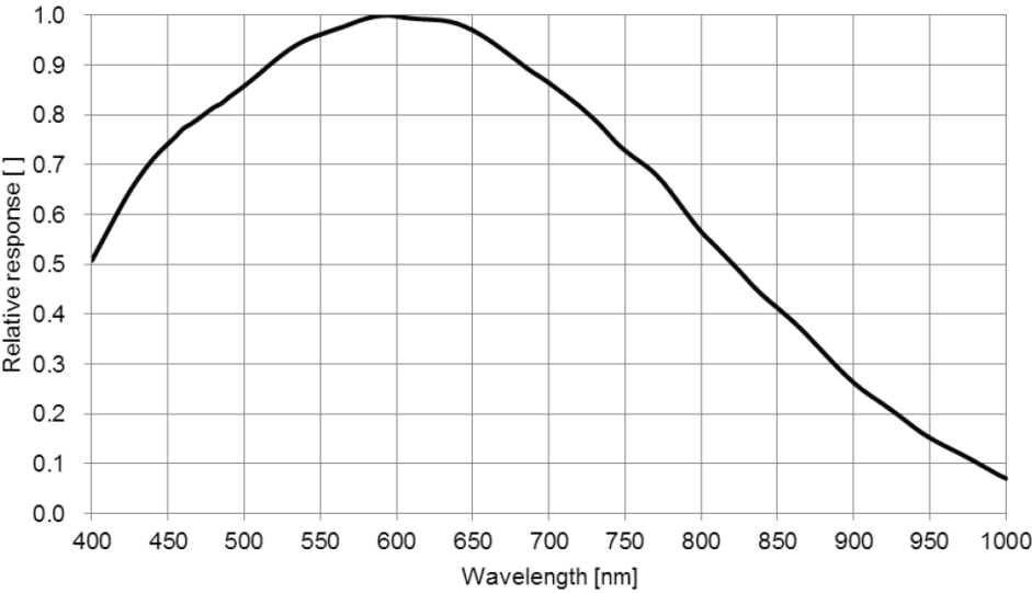
Figure 5-64 I3CMOS05000KMB spectral response curve
