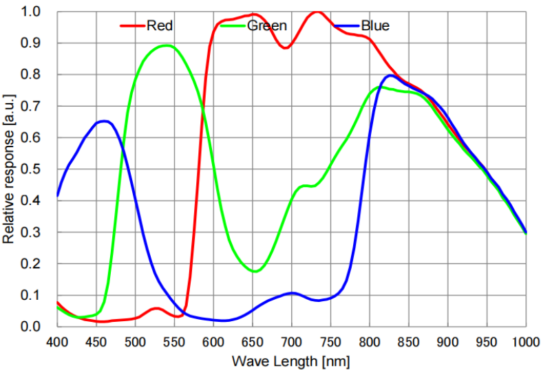
Figure 3-16 ITR3CMOS08300KPA spectral response curve
