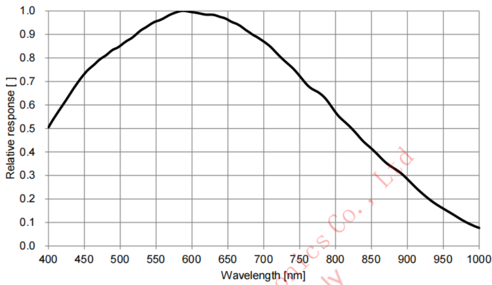
Figure 5-81 I3CMOS01700KMB spectral response curve
