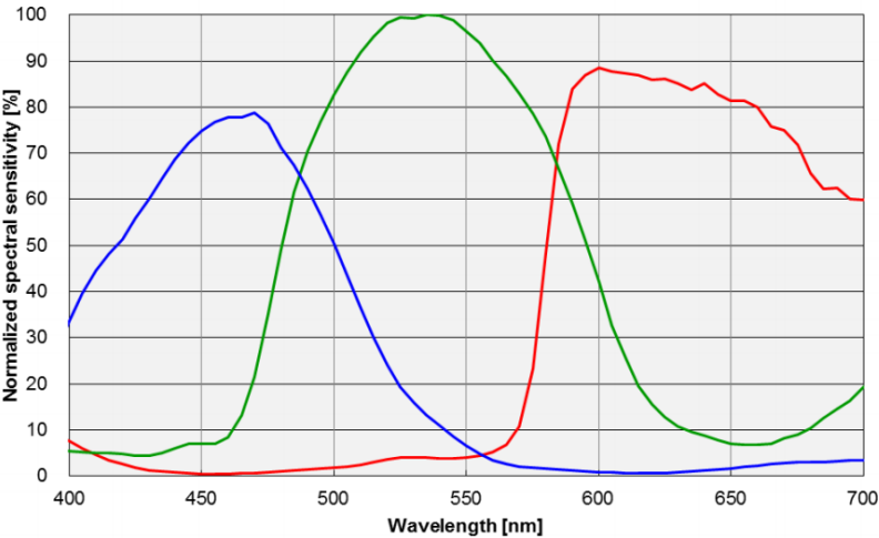
Figure 2-12 MAX102AC-10G spectral response curve
