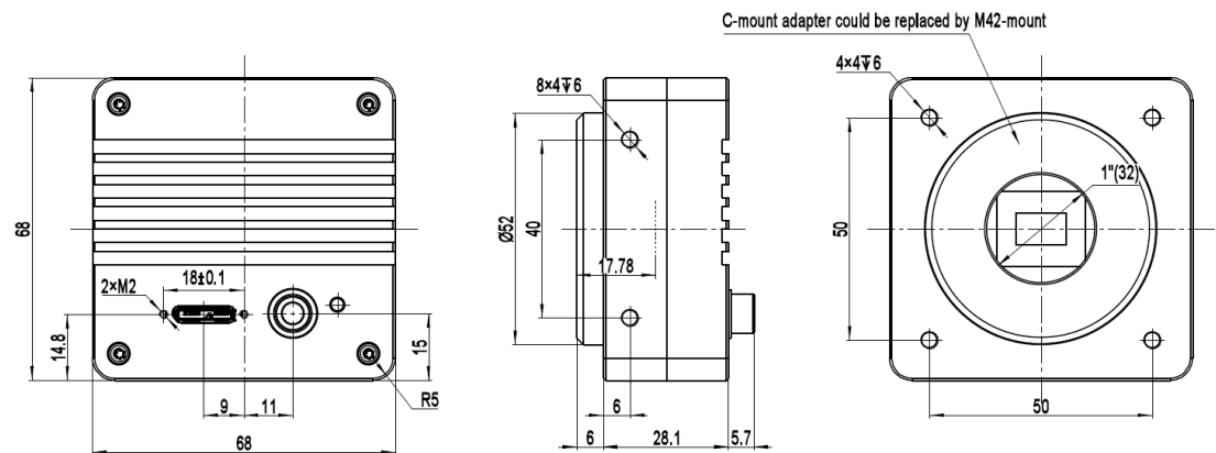
Figure 12-31 Dimensions of IUA camera housing (mm)
