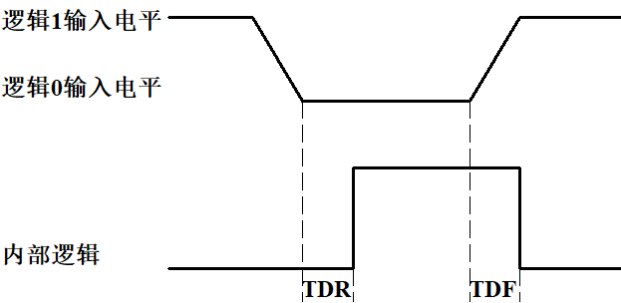
Figure 13-14 Input logic level
