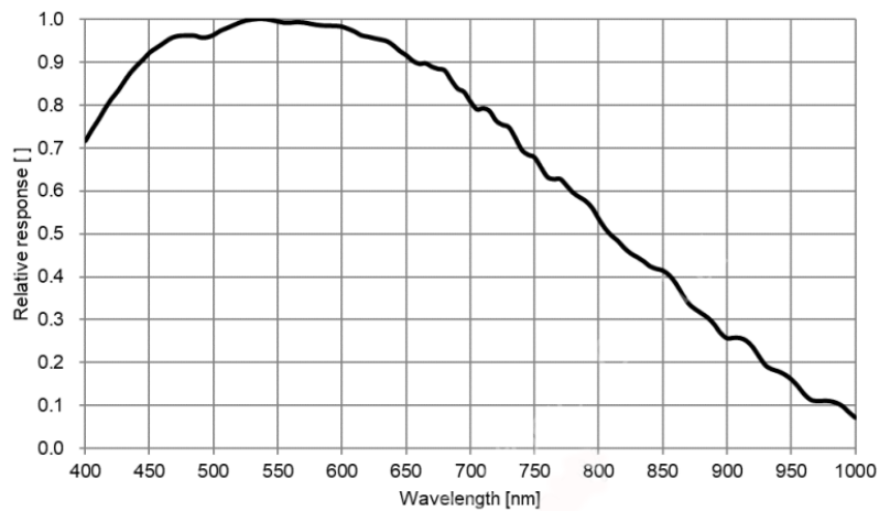
Figure 5-74 I3CMOS05100KMB-CXP spectral response curve
