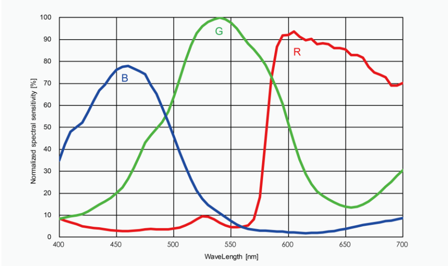
Figure 8-6 IUC21000KPA spectral response curve
