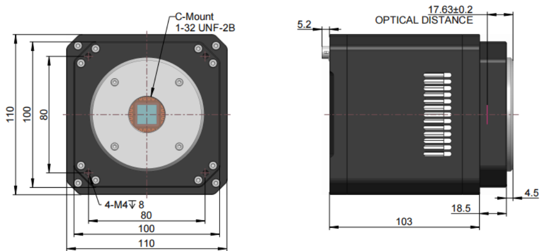
Figure 12-4 MAX04AM& MAX04AM dimensions (mm)
