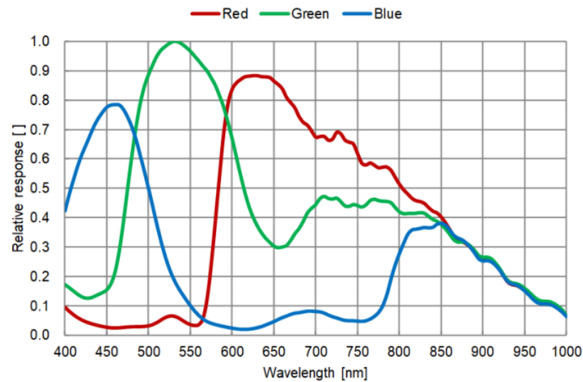
Figure 6-42 IUA8000KPB spectral response curve
