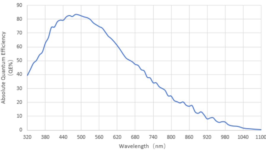
Figure 6-34 IUA6300KMA absolute quantum efficiency
