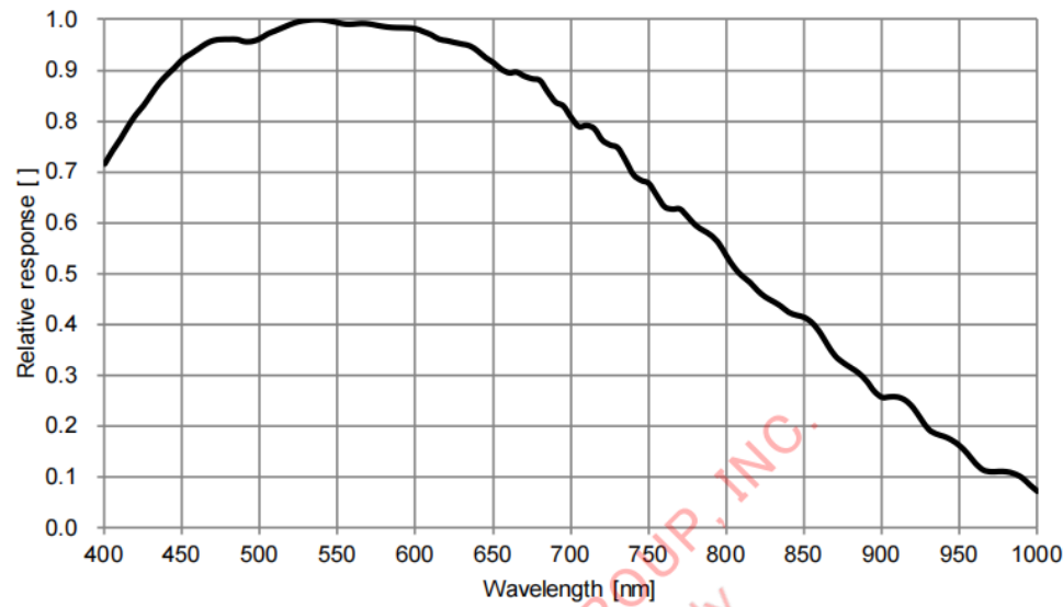
Figure 5-77 I3CMOS08000KMA spectral response curve
