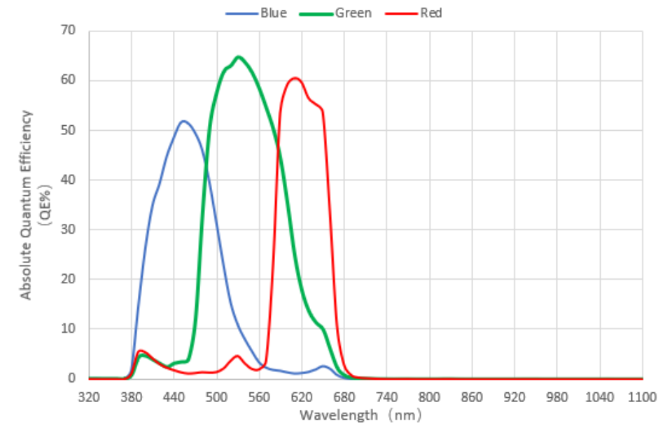
Figure 6-32 IUA5100KPA absolute quantum efficiency
