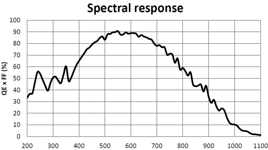
Figure 3-26 ITR3CMOS00500KMA spectral response curve
