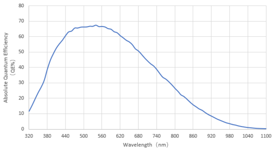
Figure 5-65 I3CMOS05000KMB absolute quantum efficiency
