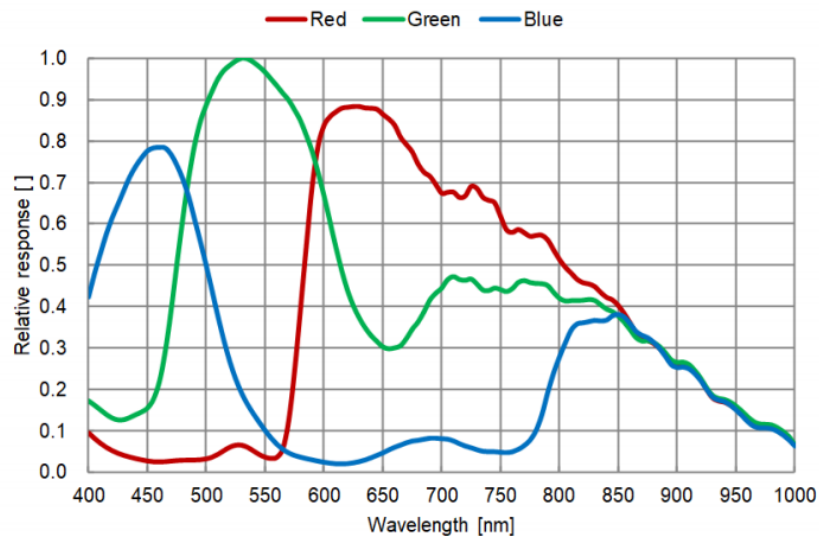
Figure 5-26 I3ISPM08000KPA spectral response curve
