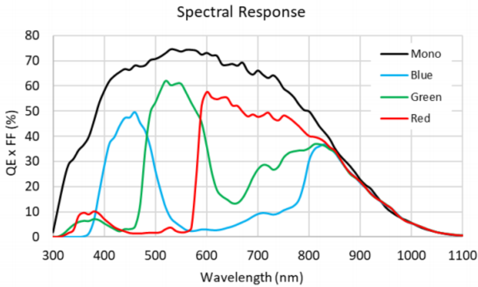
Figure 5-52 I3CMOS02400KMA spectral response curve
