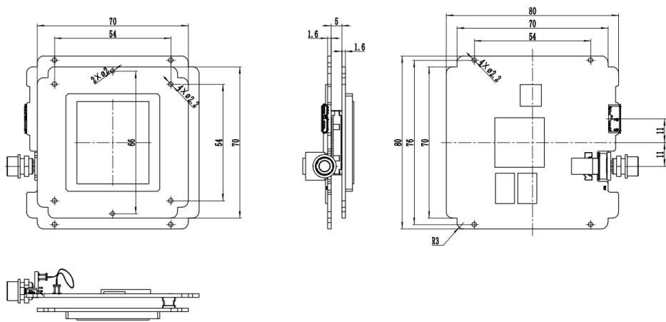
Figure 12-38 Dimensions of IUC circuit board (mm)
