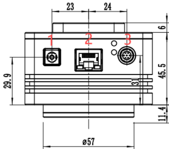
Figure 12-18 CTR3CMOS Camera interface diagram
