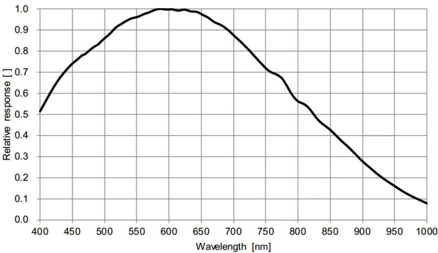
Figure 5-47 I3CMOS00500KMA spectral response curve
