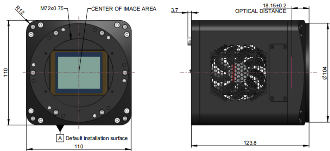
Figure 12-2 MAX102 dimensions (mm)
