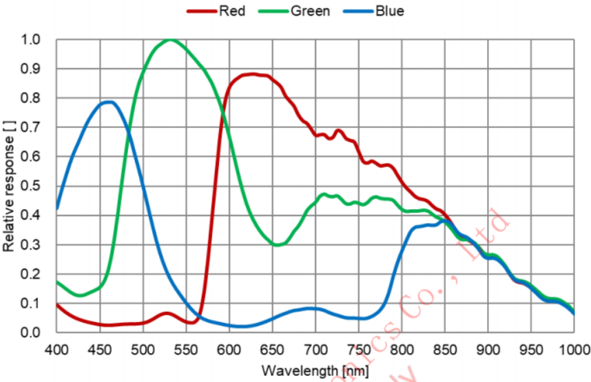
Figure 5-45 I3ISPM20400KPA spectral response curve
