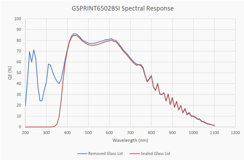
Figure 5-46 I3CMOS02000KMB spectral response curve
