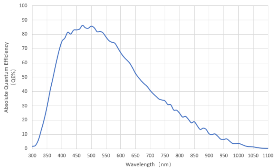
Figure 4-30 CTR3CMOS45000KMA spectral absolute quantum efficiency
