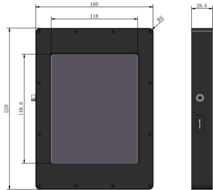
Figure 12-46 Dimensions of IUE camera housing (mm)
