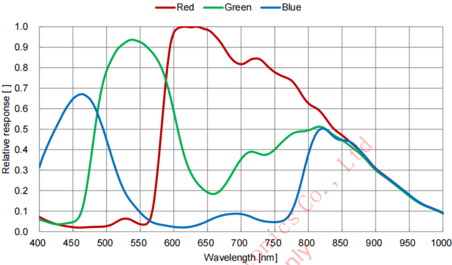
Figure 5-34 I3ISPM02000KPA spectral response curve
