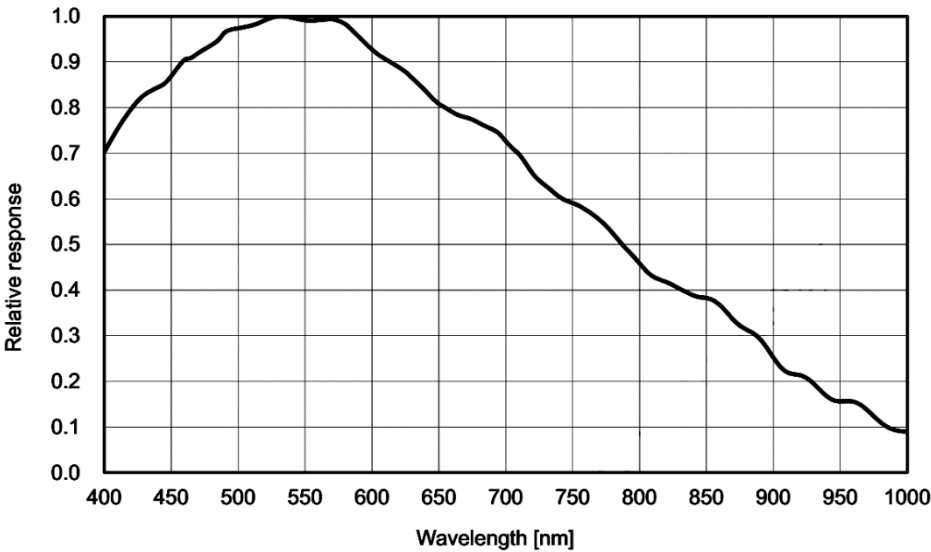
Figure 6-58 IUA20000KMA spectral response curve
