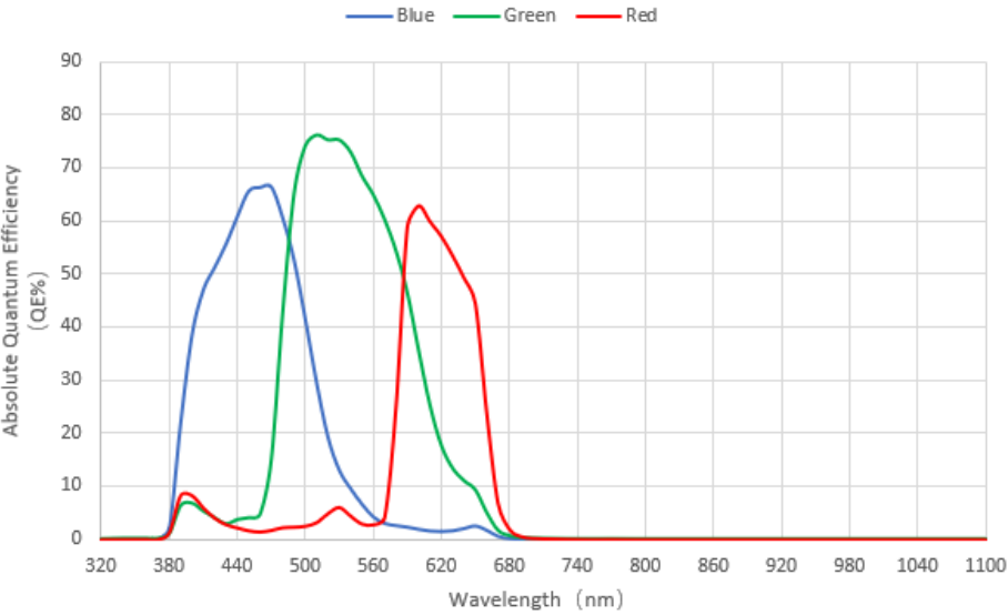
Figure 6-61 IUA20000KPA absolute quantum efficiency
