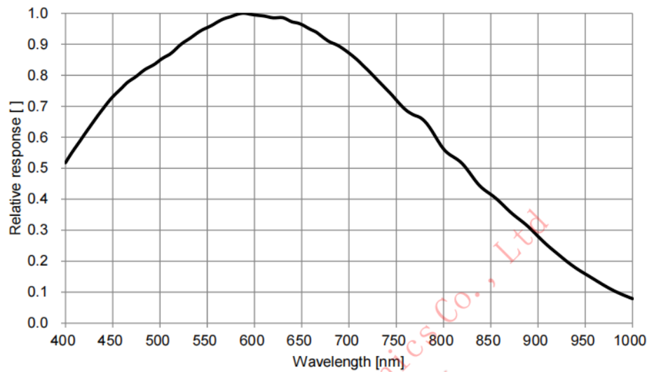
Figure 5-83 I3CMOS02000KMA spectral response curve
