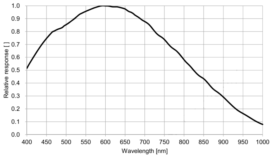
Figure 5-86 I3CMOS07100KMA spectral response curve
