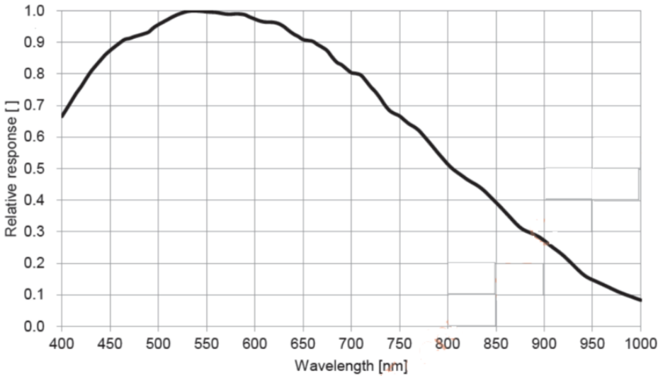
Figure 6-62 IUA20400KMA spectral response curve
