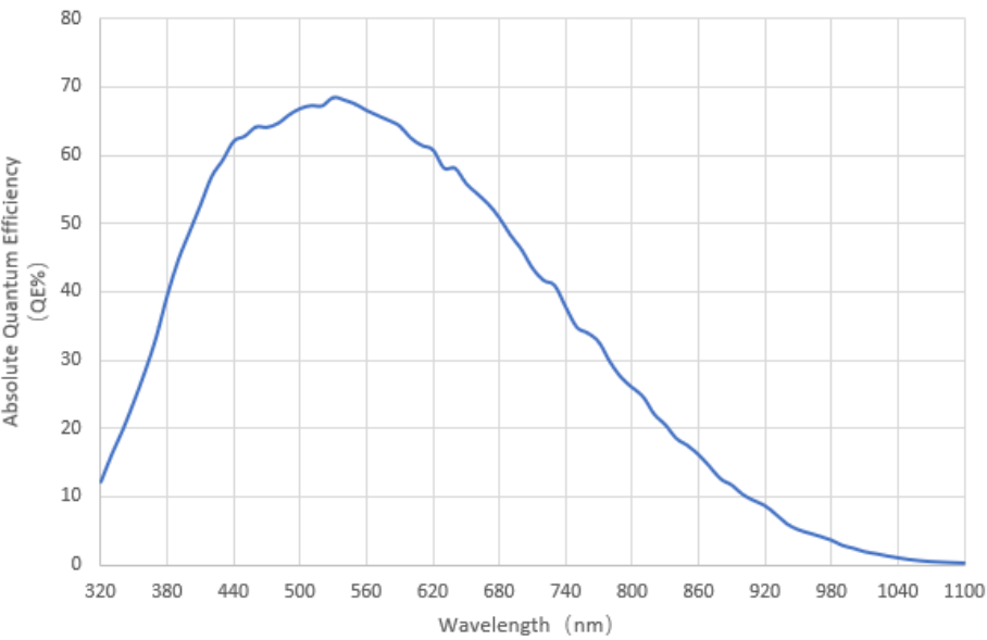
Figure 5-57 I3CMOS03100KMB-G absolute quantum efficiency
