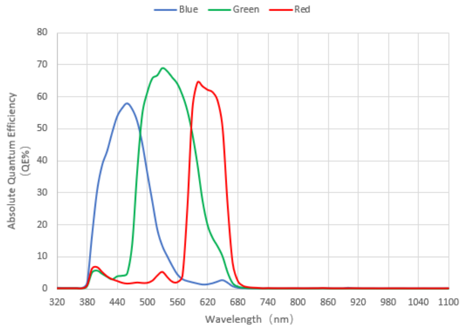
Figure 4-14 CTR3CMOS07100KPA-G spectral absolute quantum efficiency
