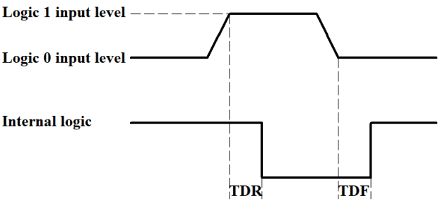
Figure 13-7 Input logic level
