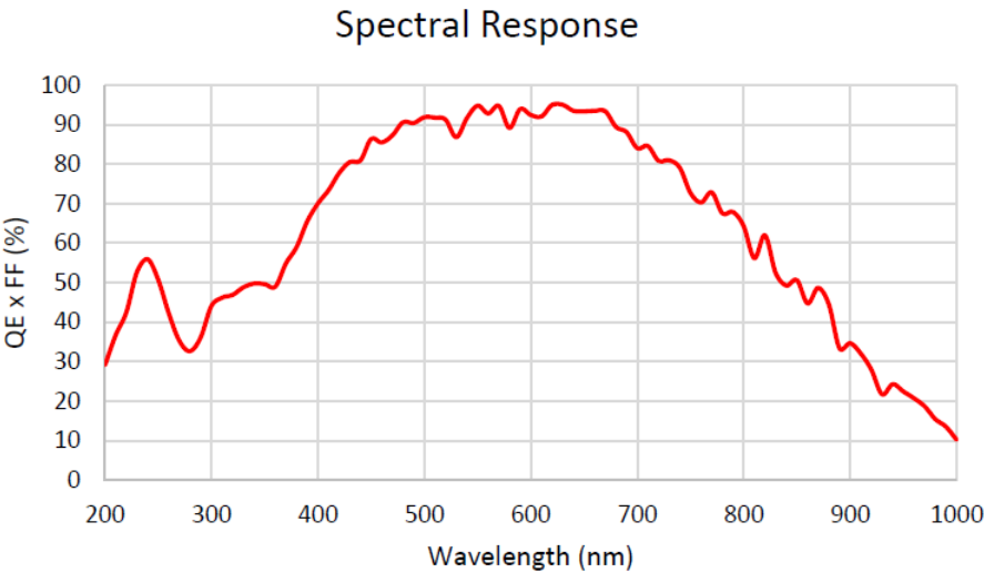
Figure 6-85 IUA4200KME spectral response curve
