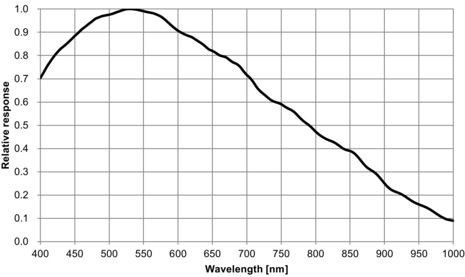
Figure 5-75 I3CMOS06300KMA spectral response curve
