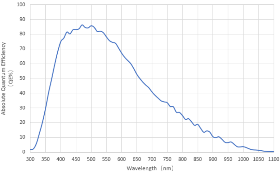
Figure 3-2 ITR3CMOS45000KMA spectral absolute quantum efficiency
