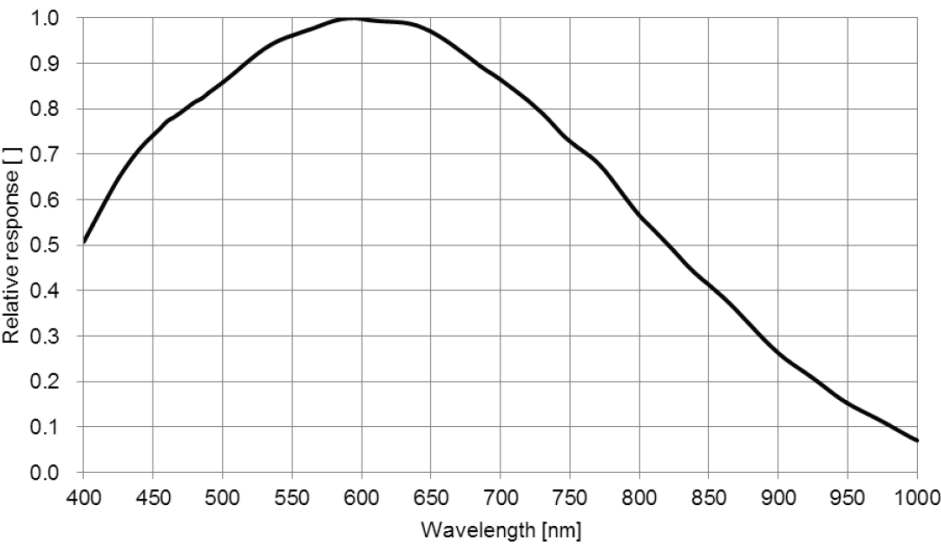
Figure 5-55 I3CMOS03100KMA-10G spectral response curve
