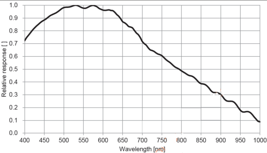
Figure 3-11 ITR3CMOS10300KMA spectral response curve
