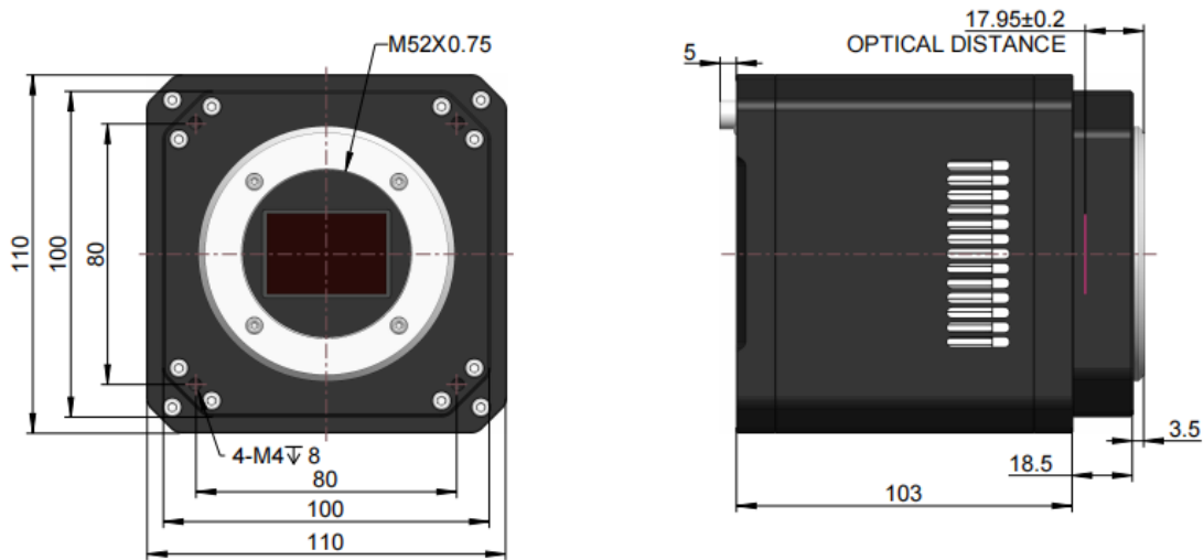
Figure 12-3 MAX62& MAX24 dimensions (mm)
