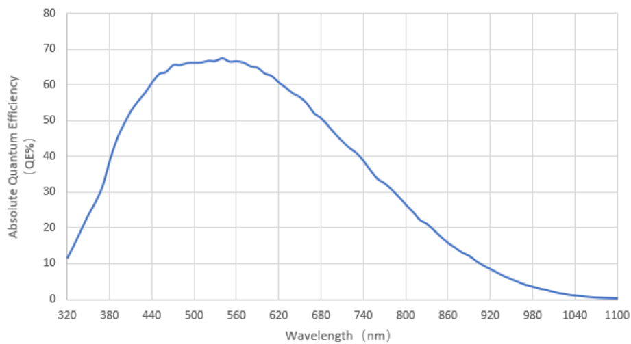
Figure 5-67 I3CMOS05000KMB-G absolute quantum efficiency
