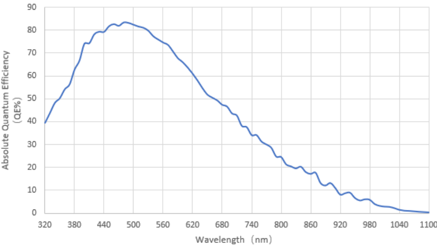
Figure 5-76 I3CMOS06300KMA absolute quantum efficiency
