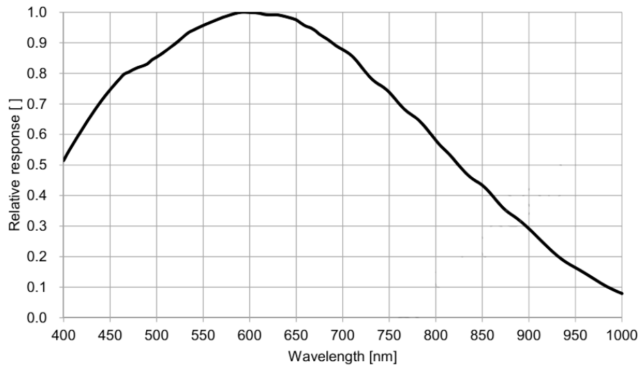
Figure 5-84 I3CMOS02800KMA spectral response curve
