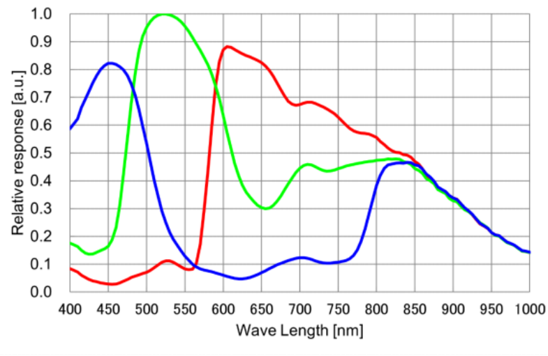
Figure 5-15 I3ISPM03200KPA spectral response curve
