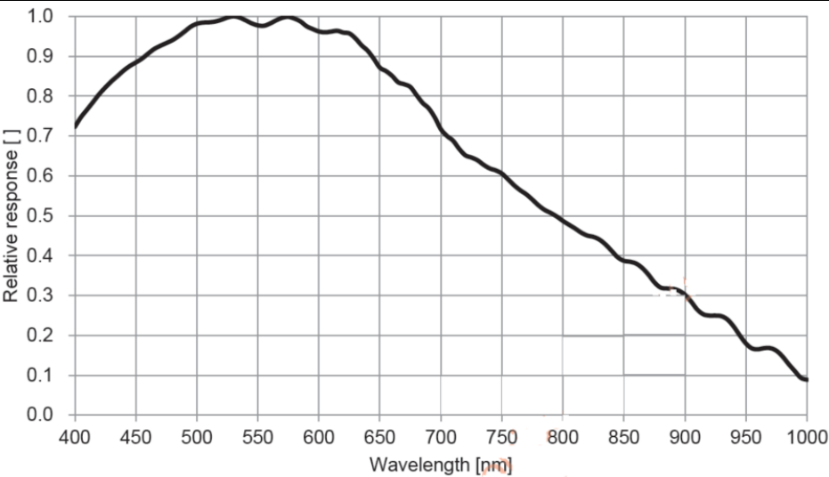
Figure 4-29 CTR3CMOS45000KMA spectral response curve
