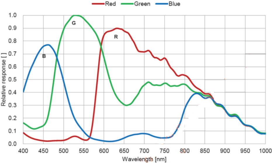
Figure 6-68 IUA24500KPA spectral response curve
