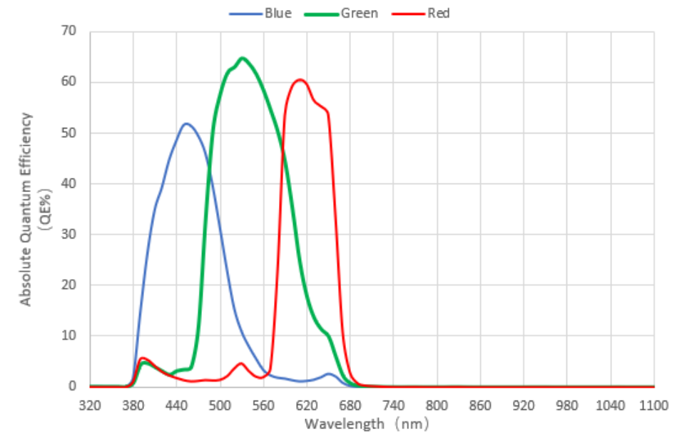
Figure 6-53 IUA12300KPA absolute quantum efficiency
