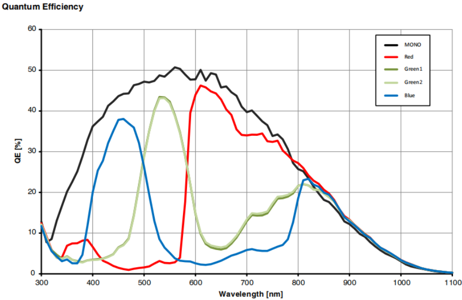
Figure 9-1 IUD16000KMA spectral response curve
