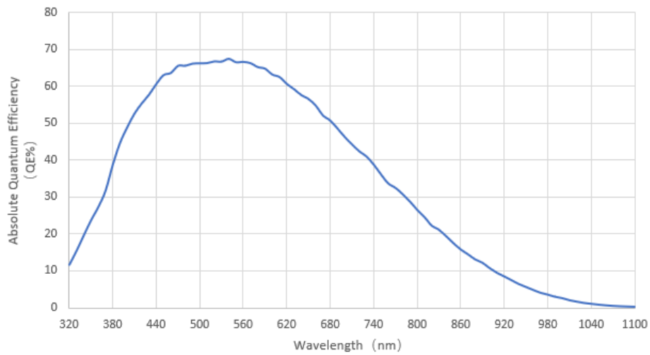
Figure 5-89 I3CMOS12300KMA absolute quantum efficiency
