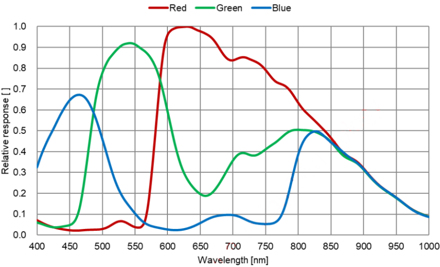
Figure 6-13 IUA1700KPA spectral response curve
