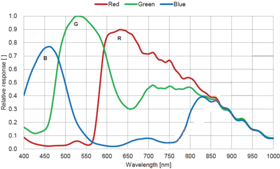
Figure 8-2 IUC20400KPA-10G spectral response curve
