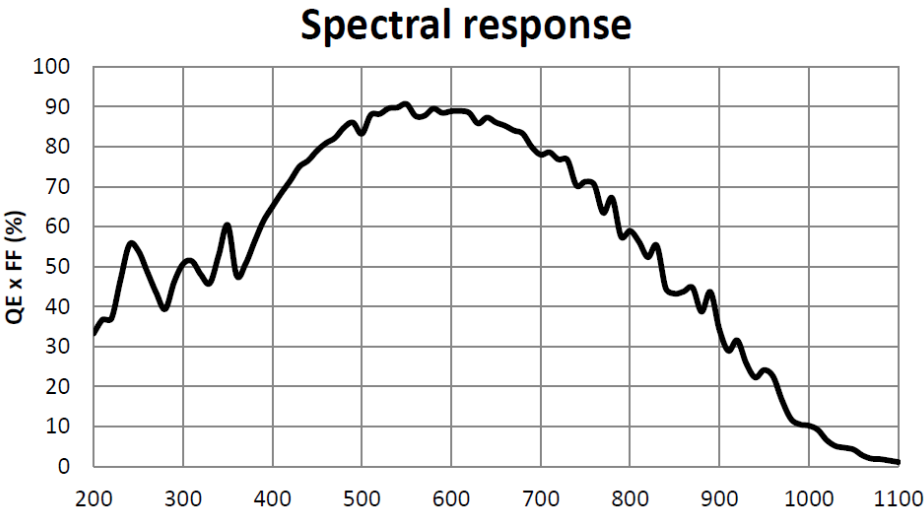
Figure 6-77 IUA5000KMA spectral response curve
