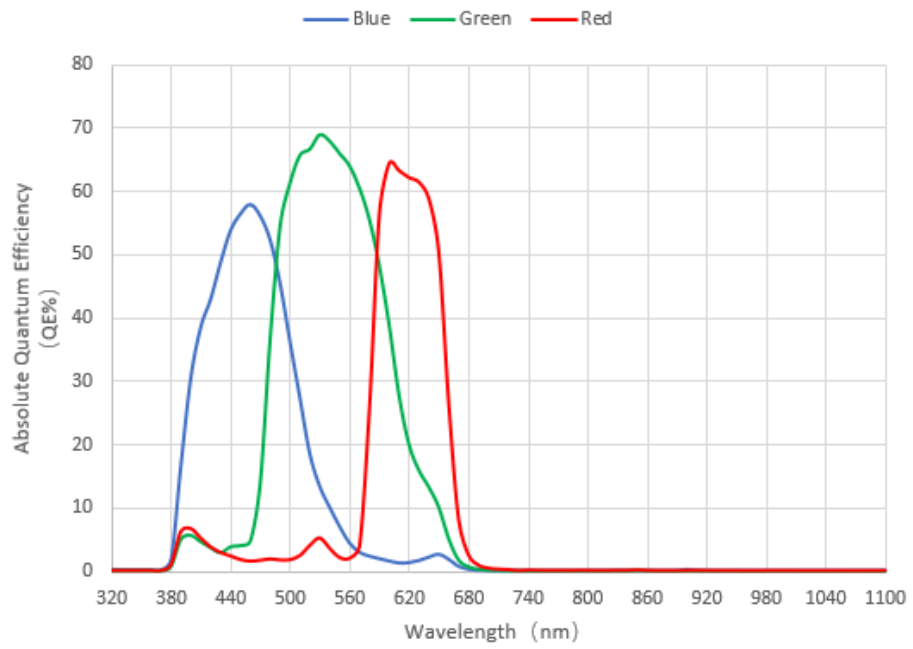
Figure 5-40 I3ISPM07100KPA absolute quantum efficiency
