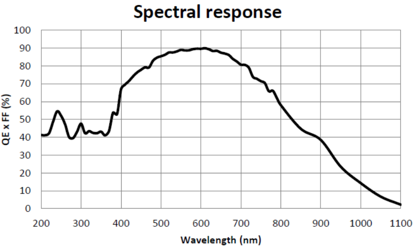
Figure 5-78 I3CMOS01300KMA spectral response curve
