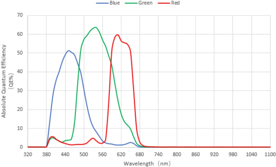
Figure 5-3 I3ISPM01500KPA absolute quantum efficiency
