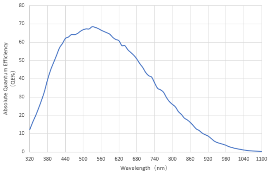
Figure 5-59 I3CMOS03100KMB absolute quantum efficiency
