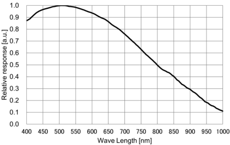
Figure 5-61 I3CMOS03200KMA spectral response curve
