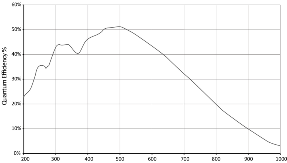
Figure 6-87 IUA8000KMA absolute quantum efficiency
