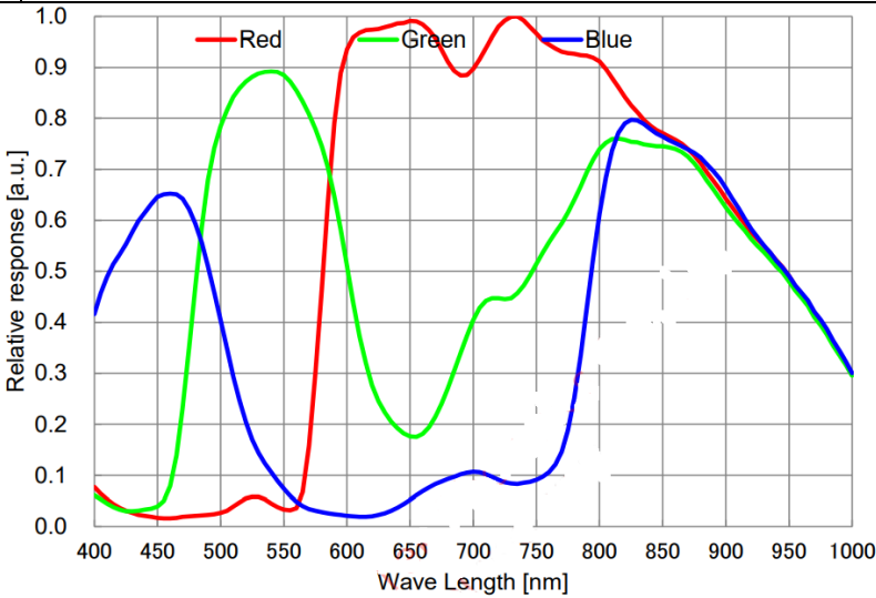
Figure 5-28 I3ISPM08300KPB spectral response curve
