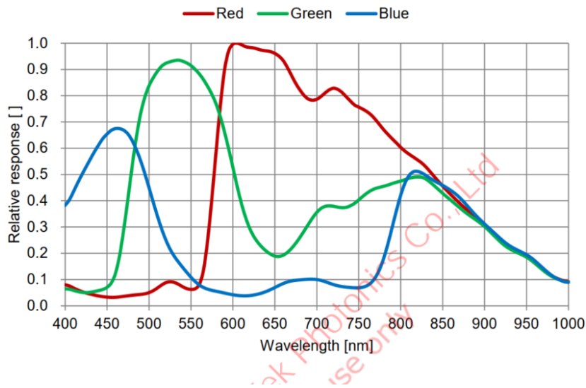
Figure 5-4 I3ISPM02000KPB spectral response curve
