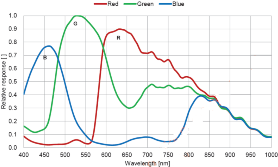
Figure 6-64 IUA20400KPA spectral response curve
