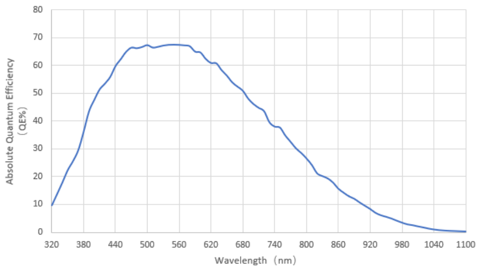
Figure 5-54 I3CMOS03100KMA absolute quantum efficiency
