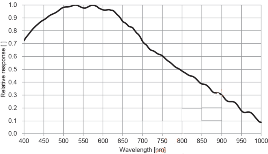
Figure 3-1 ITR3CMOS45000KMA spectral response curve
