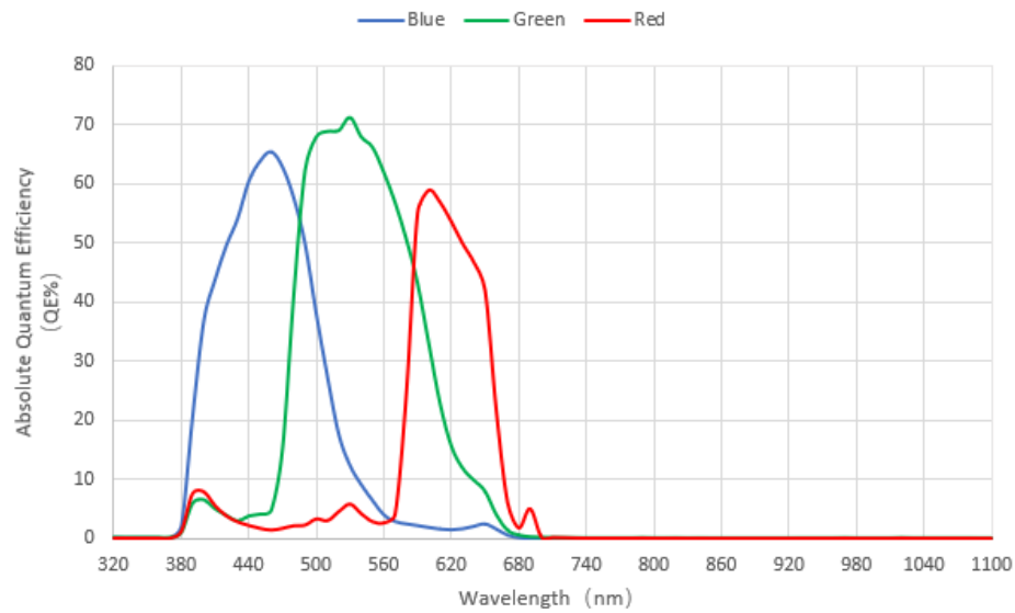
Figure 6-36 IUA6300KPA absolute quantum efficiency
