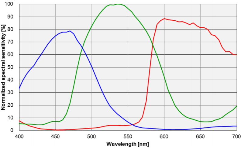
Figure 2-11 MAX102AC-U3 spectral response curve
