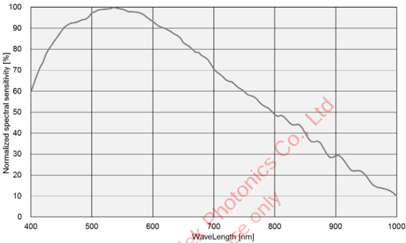
Figure 2-2 MAX251AM-10G spectral response curve
