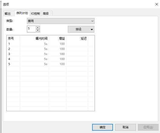
Figure 15-4 Options>Sequence page
