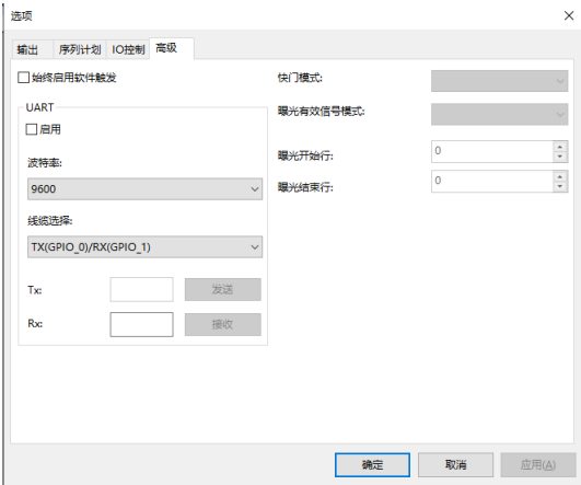
Figure 15-6 Options>Advanced page
