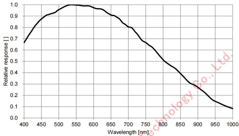
Figure 5-96 I3CMOS20400KMA spectral response curve
