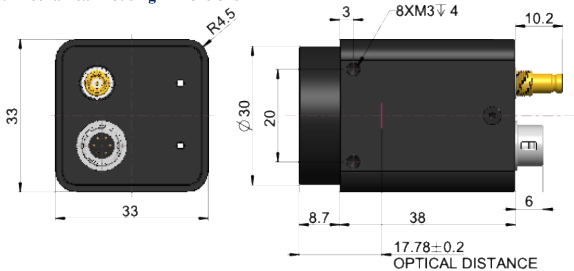
Figure 12-29 Dimensions of camera housing(mm)
