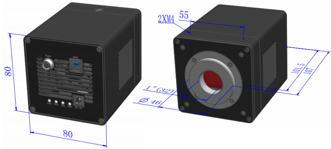
Figure 12-11 ITR3CMOS dimensions (mm)
