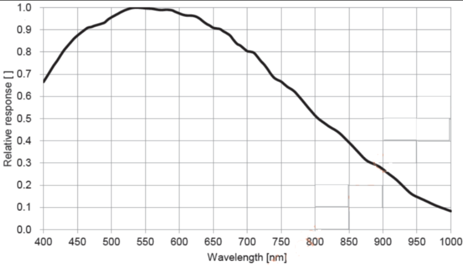
Figure 6-66 IUA24500KMA spectral response curve
