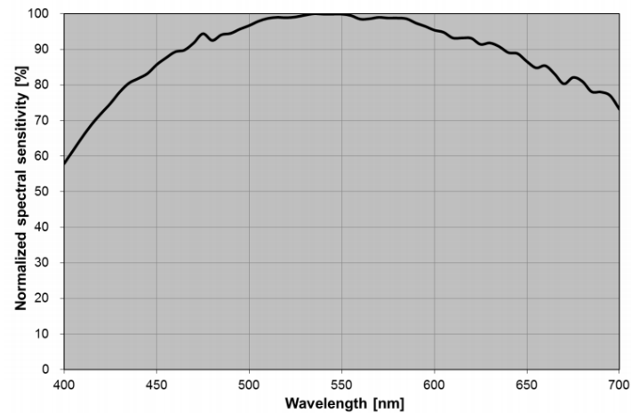
Figure 2-10 MAX102AM-10G spectral response curve
