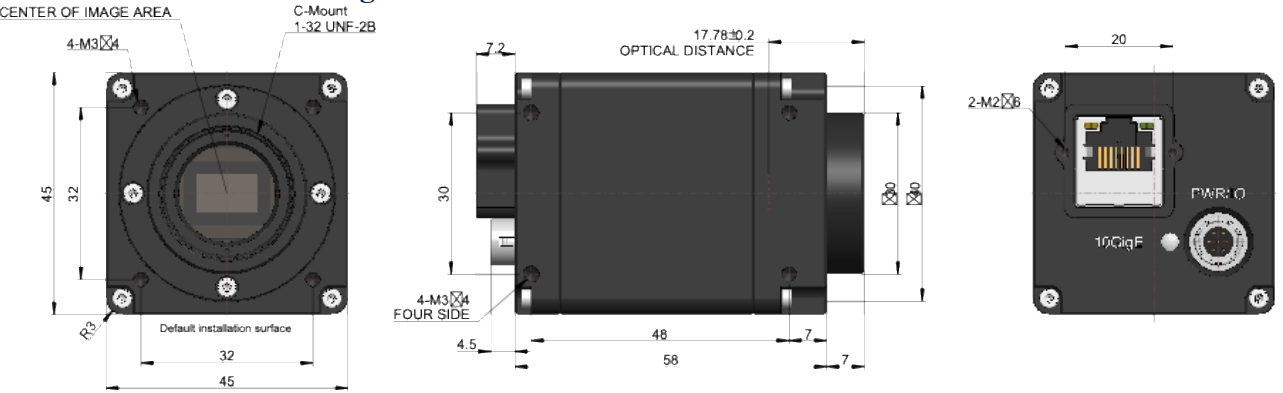
Figure 12-26 Dimensions of camera housing(mm)
