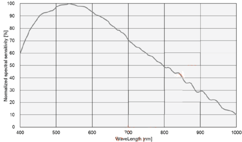
Figure 8-21 IUC60000KMA-AFU spectral response curve
