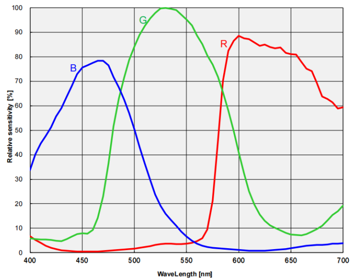
Figure 3-3 ITR3CMOS26000KPA spectral response curve
