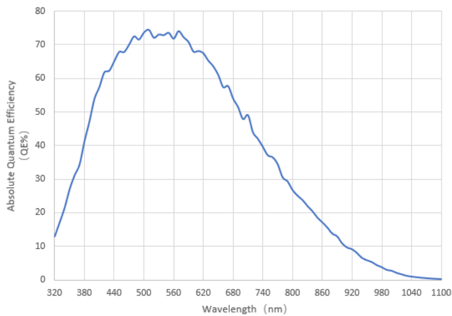
Figure 5-85 I3CMOS02800KMA absolute quantum efficiency
