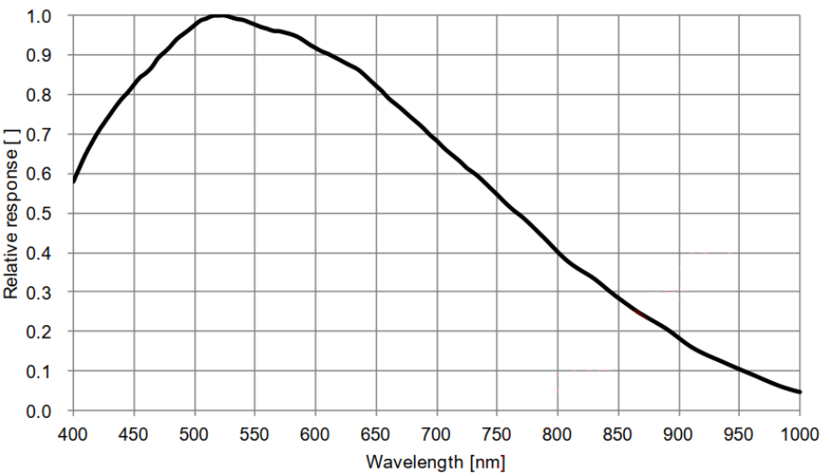
Figure 5-50 I3CMOS02300KMA spectral response curve
