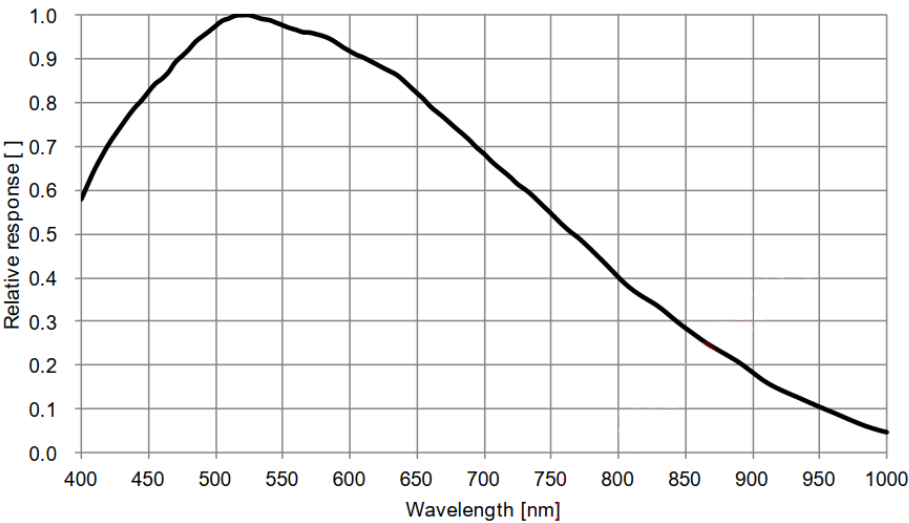
Figure 5-51 I3CMOS02300KMB spectral response curve
