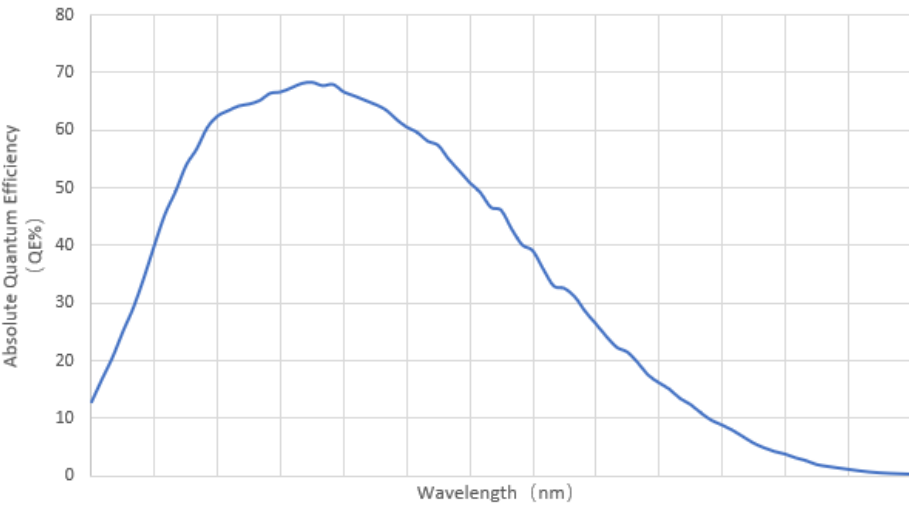
Figure 5-49 I3CMOS01500KMA absolute quantum efficiency
