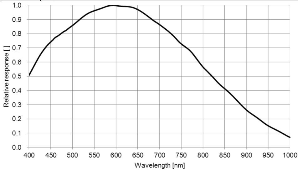
Figure 5-62 I3CMOS05000KMA spectral response curve
