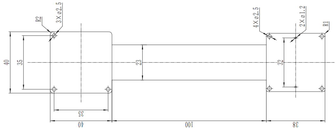
Figure 12-49 Dimensions of OEM1 circuit board (mm)
