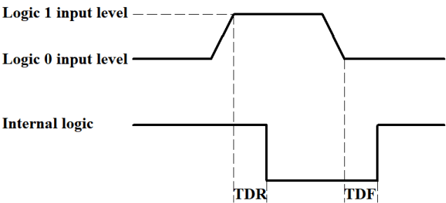
Figure 13-2 Input logic level
