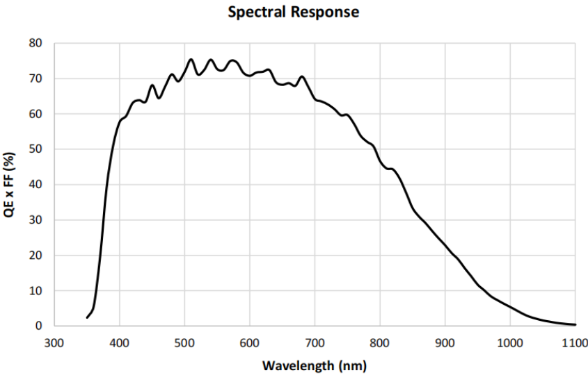
Figure 5-95 I3CMOS12500KMA spectral response curve
