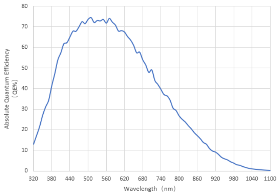
Figure 5-80 I3CMOS01700KMA absolute quantum efficiency
