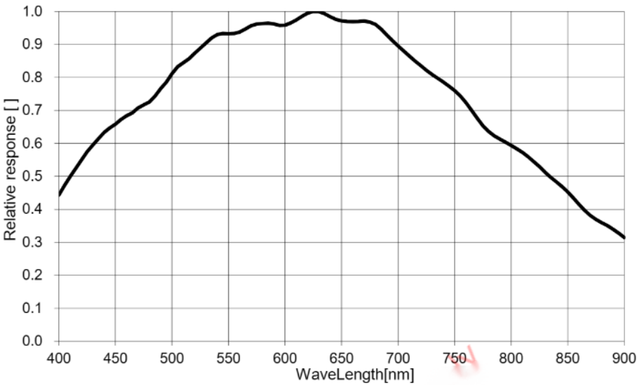
Figure 5-68 I3CMOS05000KMC spectral response curve
