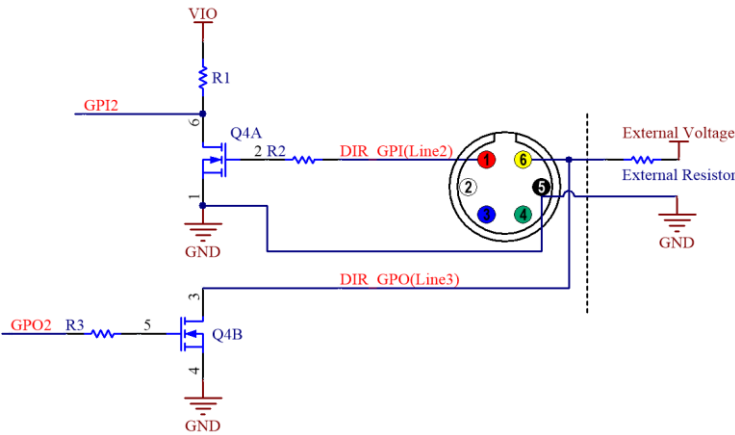
Figure 13-13 Non-isolated input, output I/ O circuit(line2)
