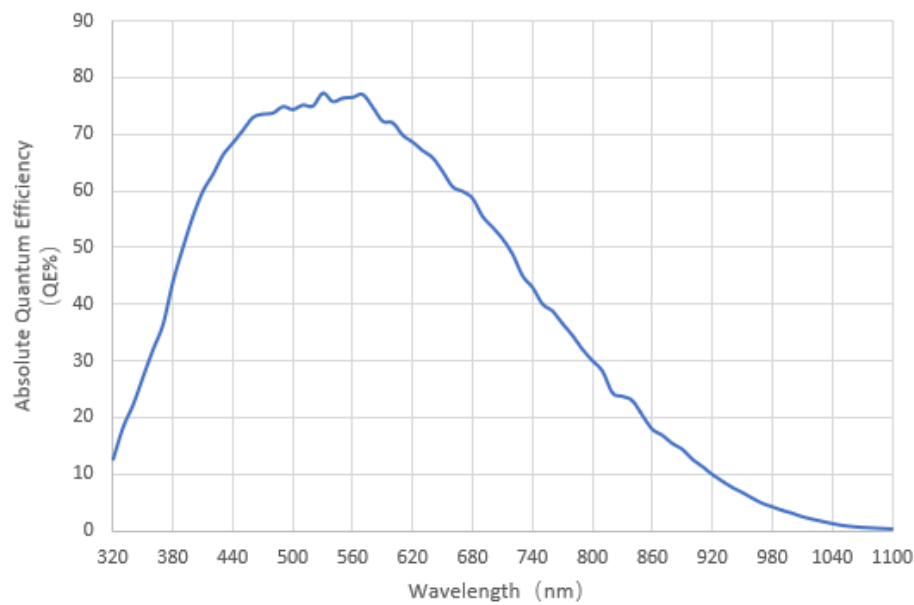
Figure 5-87 I3CMOS07100KMA absolute quantum efficiency
