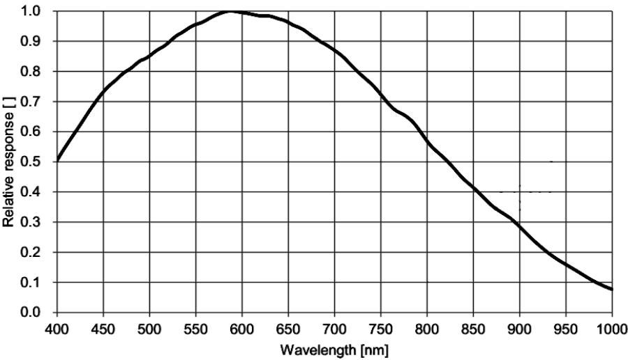
Figure 5-79 I3CMOS01700KMA spectral response curve
