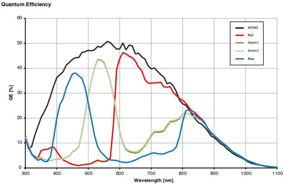
Figure 9-2 IUD25000KMA spectral response curve
