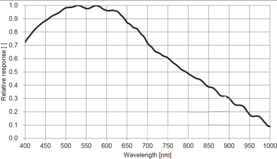
Figure 6-72 IUA45000KMA spectral response curve
