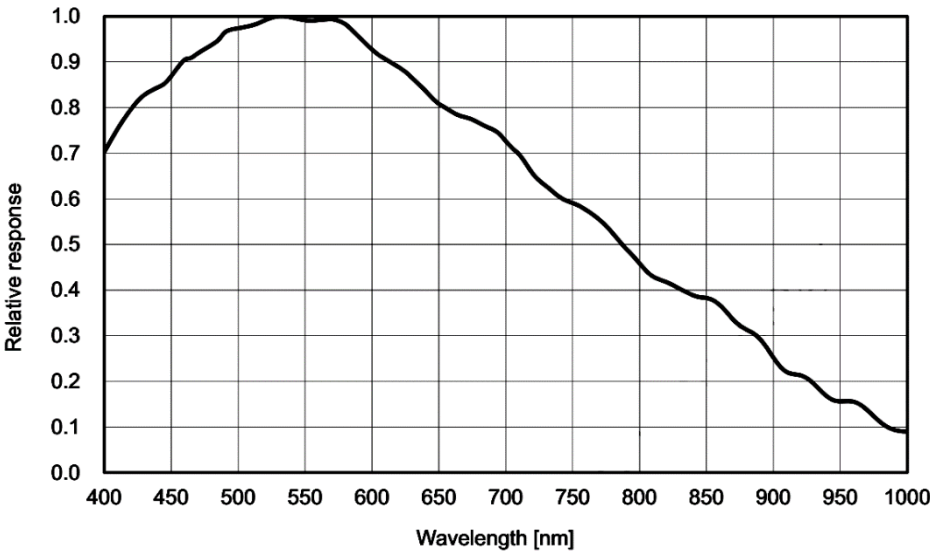
Figure 3-28 ITR3CMOS20000KMA-G spectral response curve
