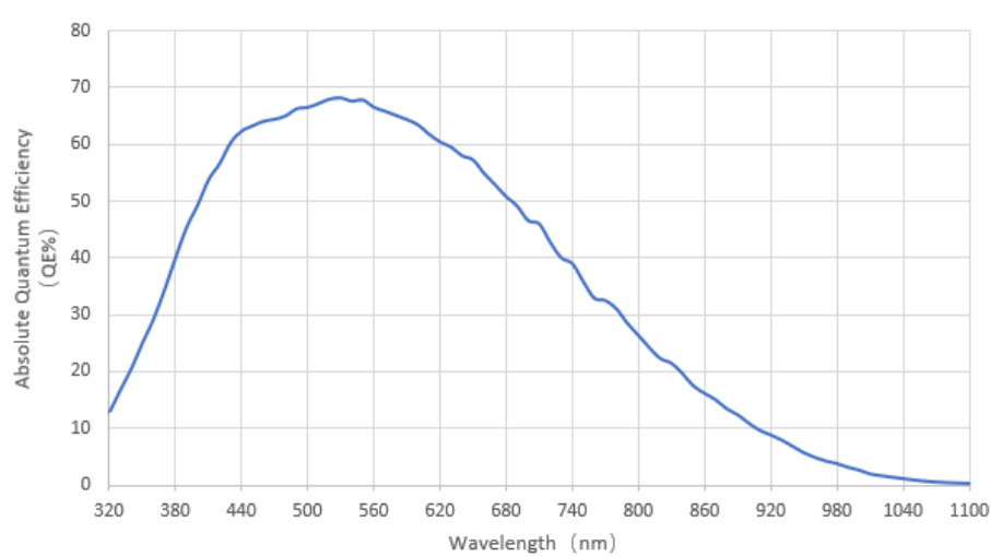
Figure 6-8 IUA1500KMA absolute quantum efficiency
