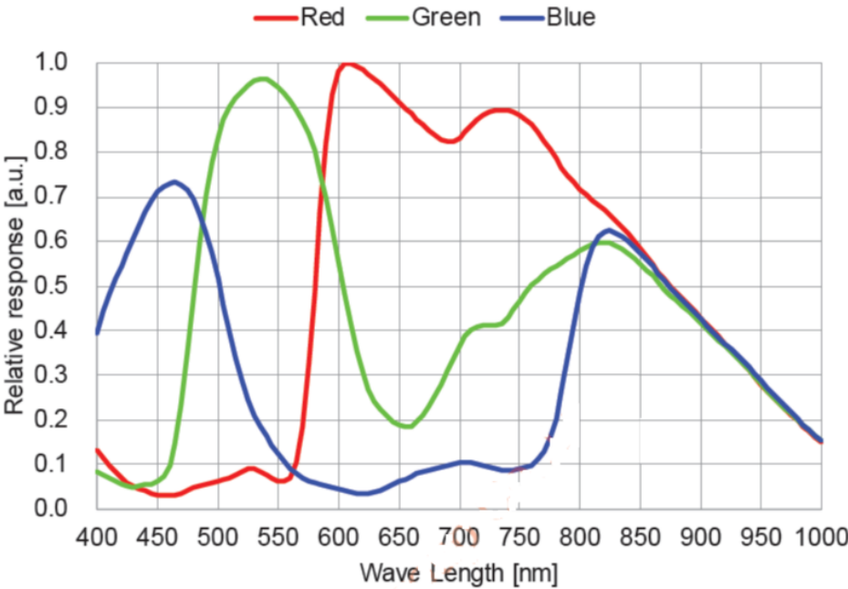
Figure 6-43 IUA8300KPA spectral response curve
