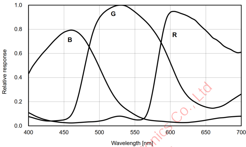
Figure 5-44 I3ISPM20000KPA spectral response curve
