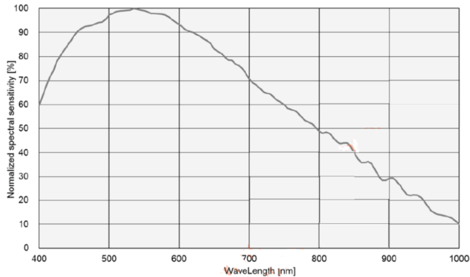
Figure 8-22 IUC60000KMA-10G spectral response curve
