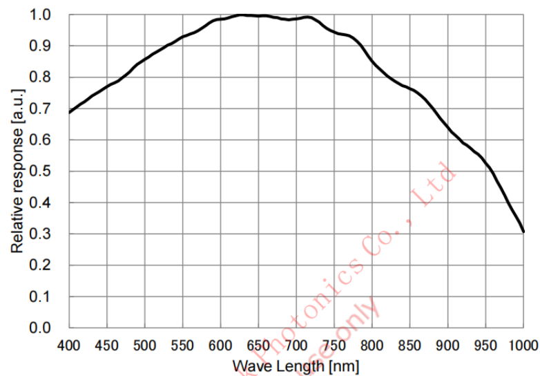
Figure 5-82 I3CMOS08300KMB spectral response curve
