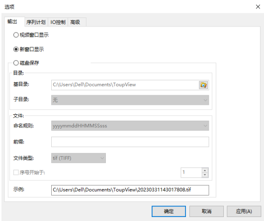
Figure 15-3 Options>Output page
