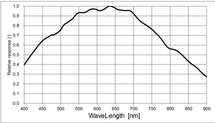
Figure 5-90 I3CMOS12300KMC spectral response curve
