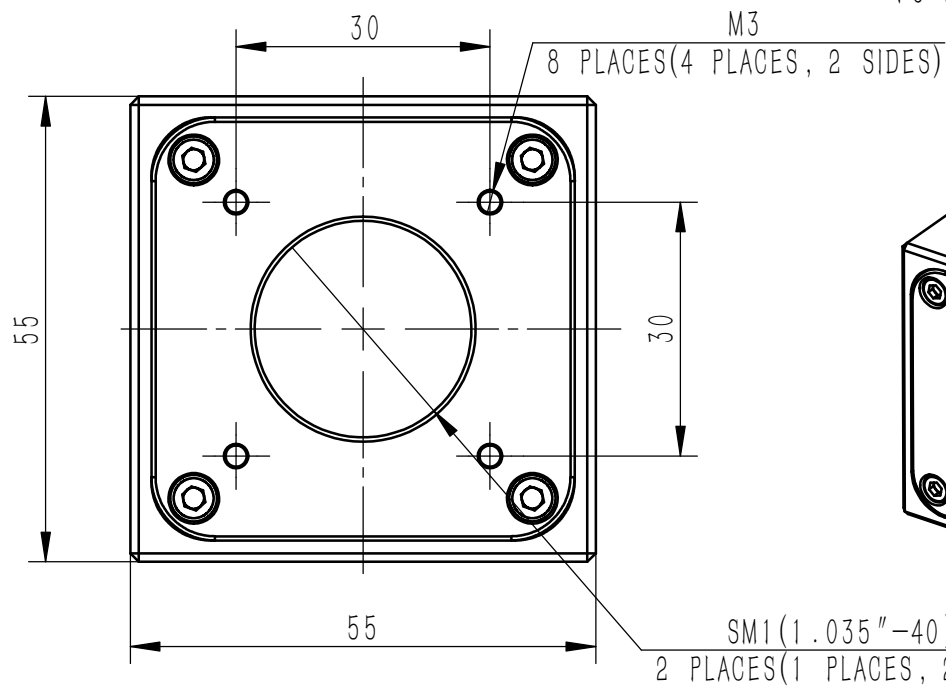
TOP AND BOTTOM VIEWS
